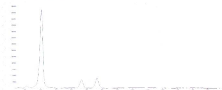
Photoluminescence
