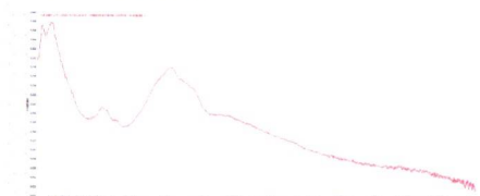
Ultraviolet-visible spectroscopy
