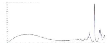
Ultraviolet-visible spectroscopy
