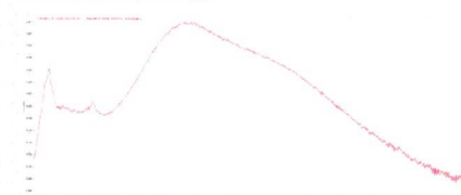
Ultraviolet-visible spectroscopy
